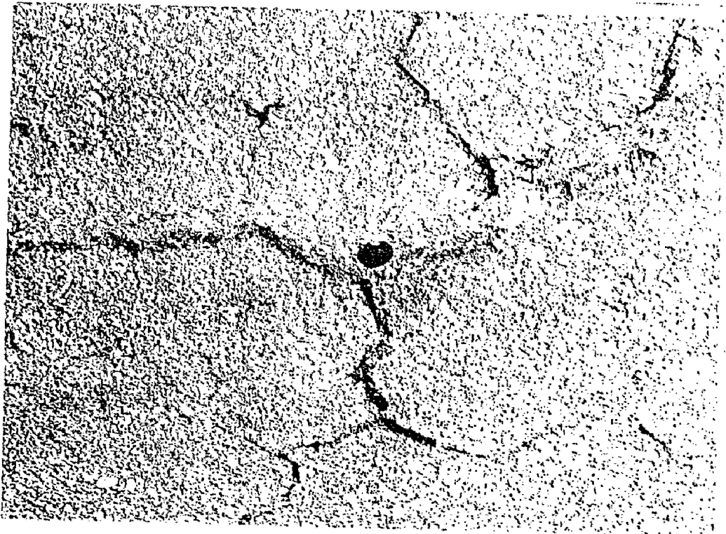
Figure 2 Cracks in the eolian deposits, east Qasr El Sagha.
