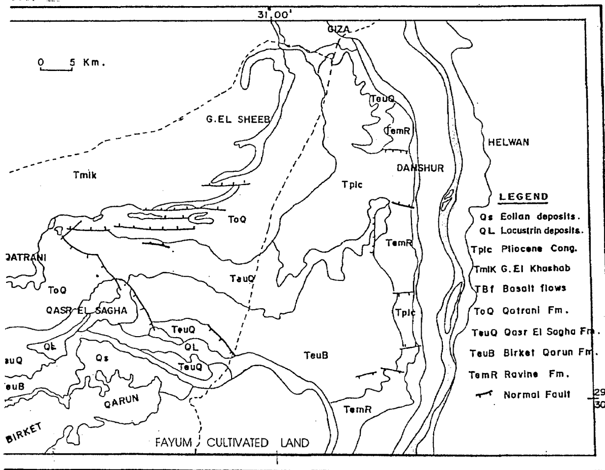
Plate III Geologic Map of Dahshour - Qatrani Area Scale 1 : 250,000
