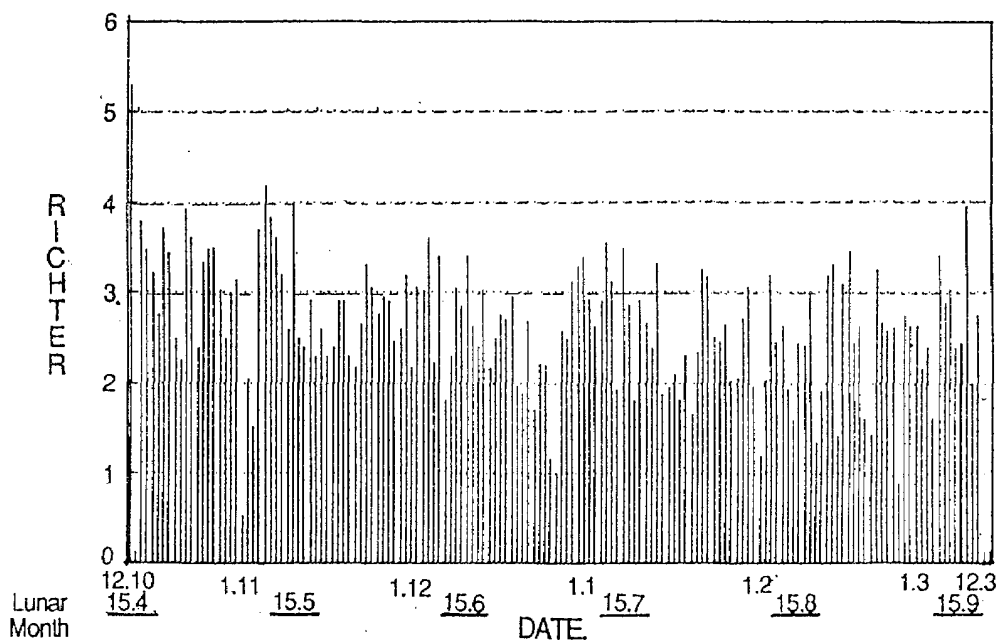
Plate IX Daily Maximum Magnitude of Dahshour Aftershocks.
