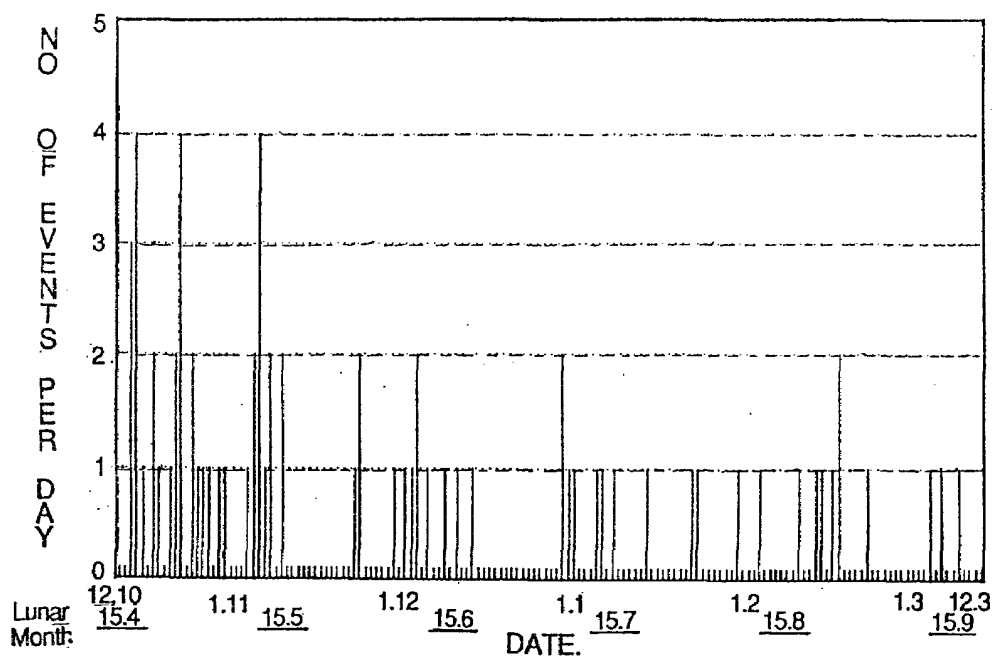
Plate X Daily Number Of Dahshour Aftershocks Greater Than Magnitude 3.
